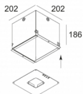
CONCRETE BOX 161 270 11 161
